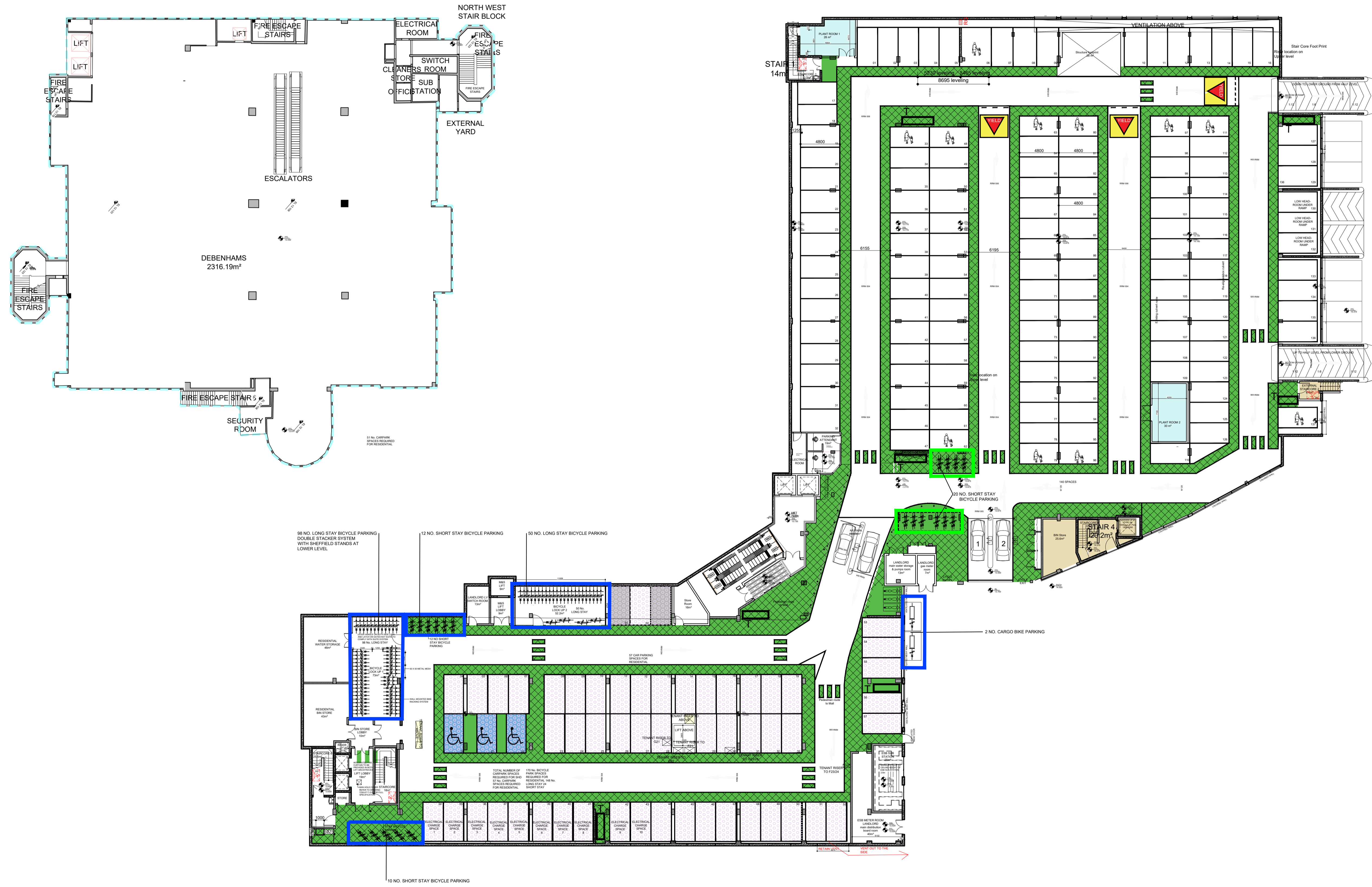
PROPOSED LOWER GROUND FLOOR BICYCLE PARKING PLAN Scale: 1:250 @ A1
